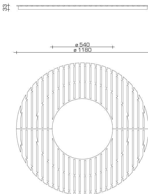
Tree grate
