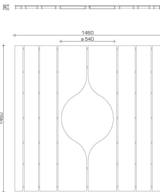
Tree grate
