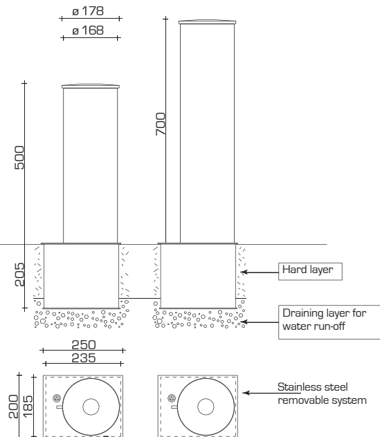
Bollards ø 178
