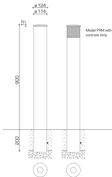
Bollard \varnothing 124
