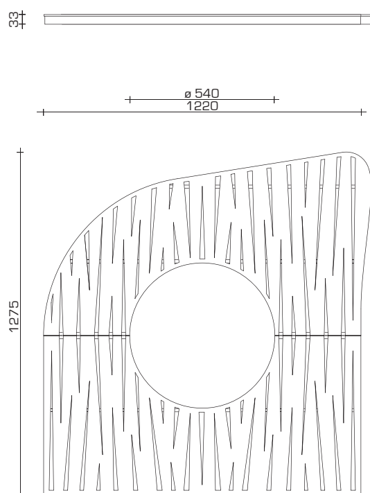
Tree grate
