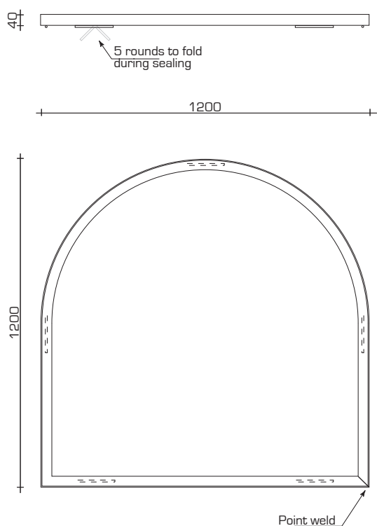
Frame
