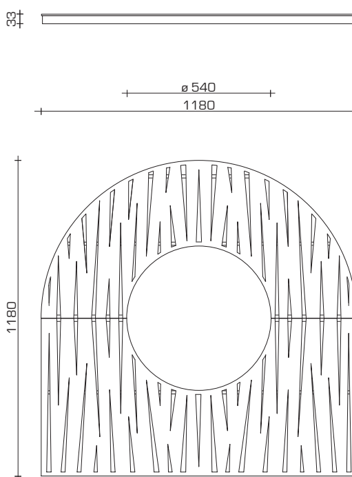
Tree grate
