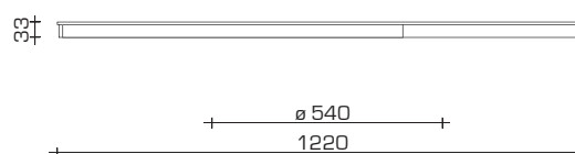
Tree grate
