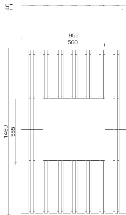
Tree grate
