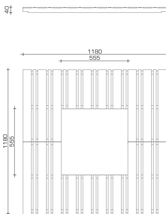
Tree grate
