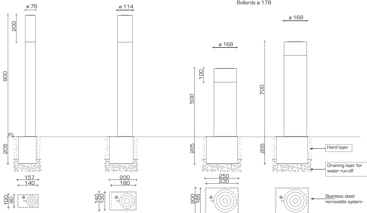
Bollards \varnothing 178
