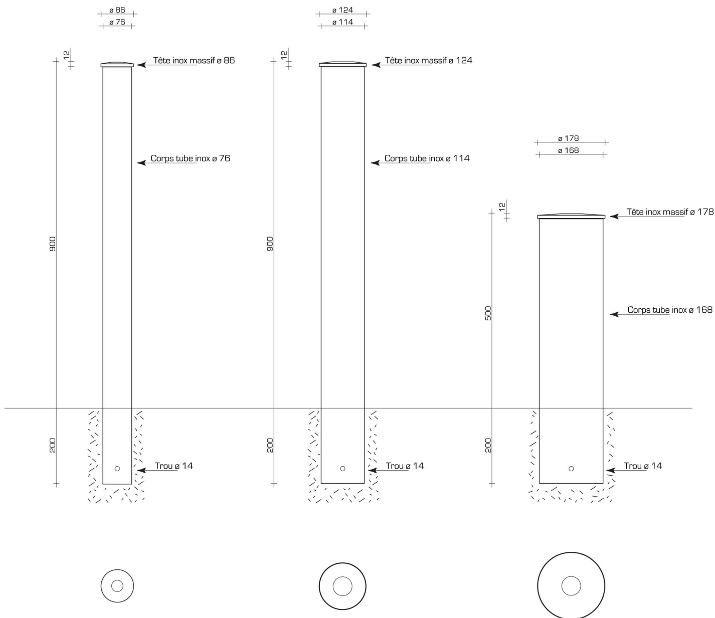
Potelet \varnothing 86
