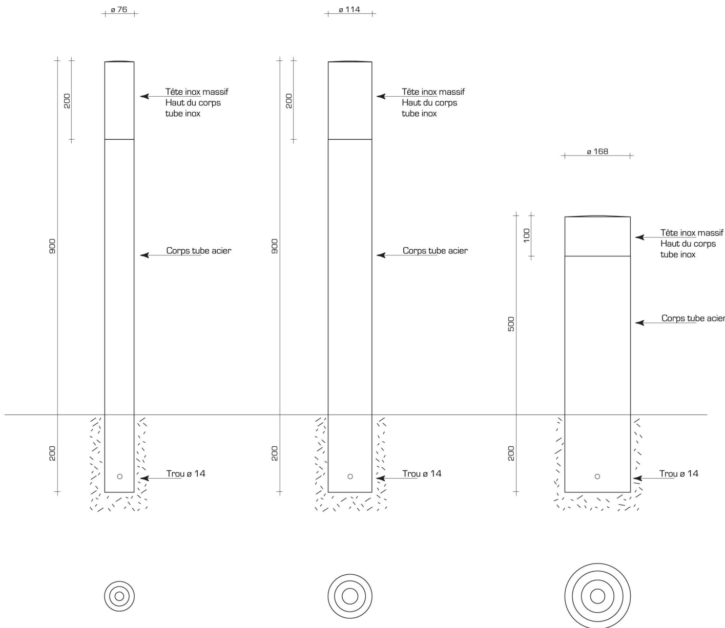
Potelet \varnothing 76
